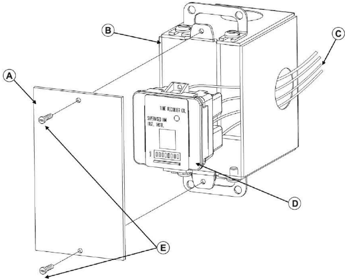
Figure 3: Mounting reference, single gang blank cover plate
