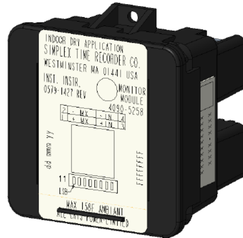
Figure 2: A4090-5258 Supervised IAM, rear view
